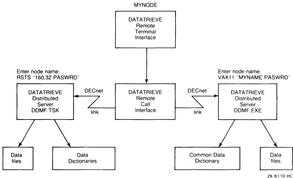
Figure 1-1: The DATATRIEVE-11 Remote Terminal Interface
