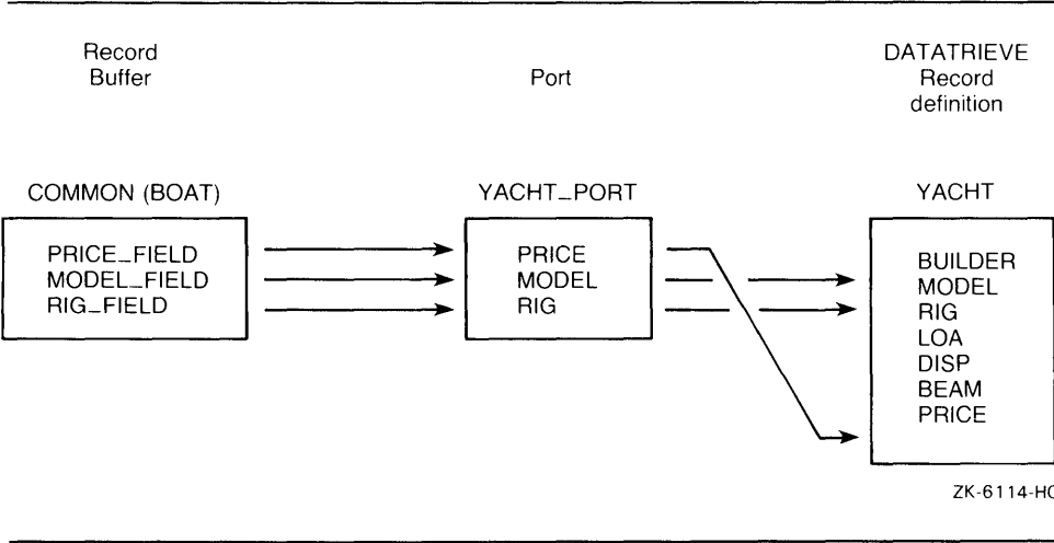
Figure 4-1: The DATATRIEVE Port
