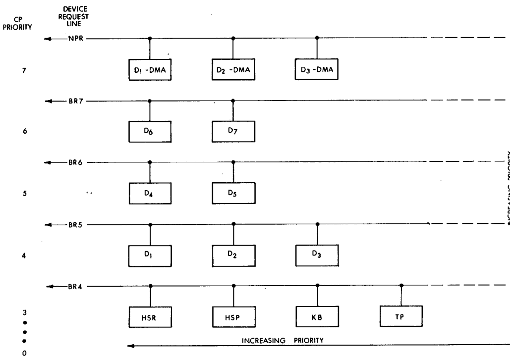
Figure 2-2 Priority Control
