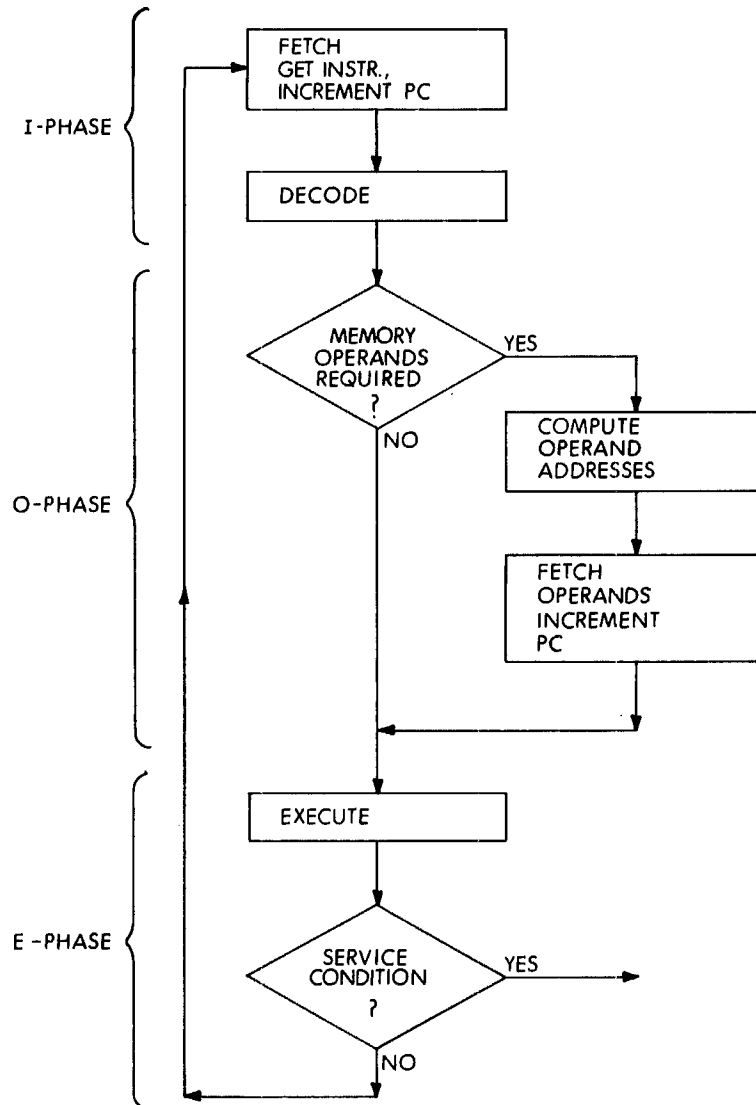
Figure 9-11 Program Flow in the PDP-11/60
