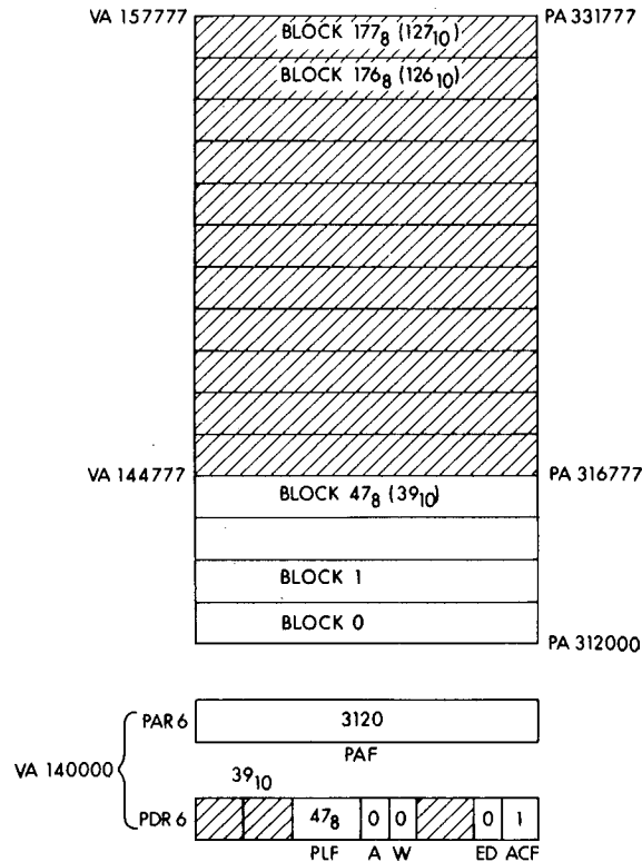
Figure 6-16 Typical Memory Page
