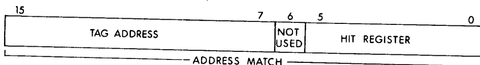
Figure 8-10 17 777 752 Cache Hit Register
