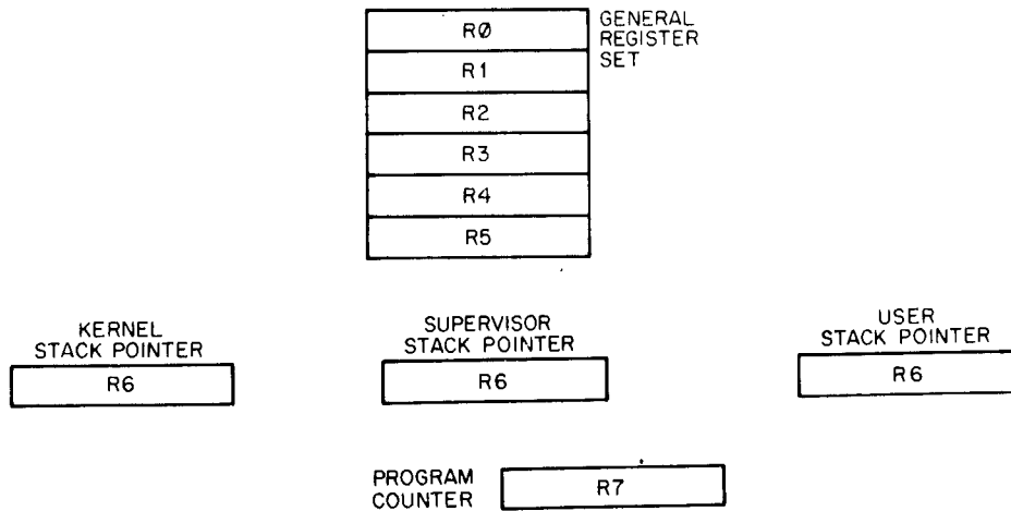
Figure 8-2 The General Registers
