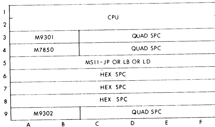
Figure 7-4 PDP-11/34A Backplane Configuration with MOS Memory
