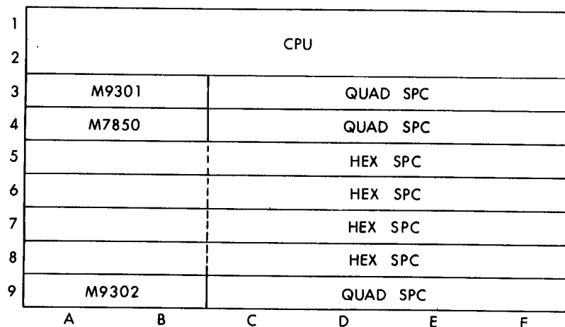
Figure 7-2 PDP-11/34A Processor Backplane Configuration
