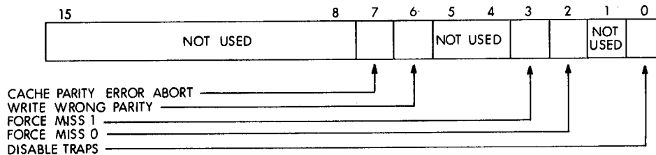
Figure 9-7 Cache Control Register 777746
