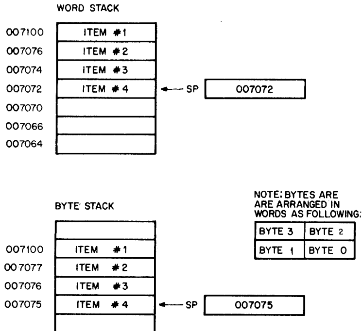
Figure 5-1 Word and Byte Stacks
