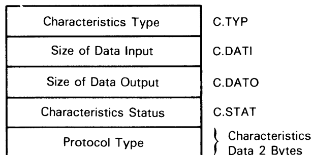
Figure 10-7: Buffer for Reading the Protocol Type
