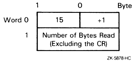
Figure 1-4: I/O Status Block for IS.xxx
